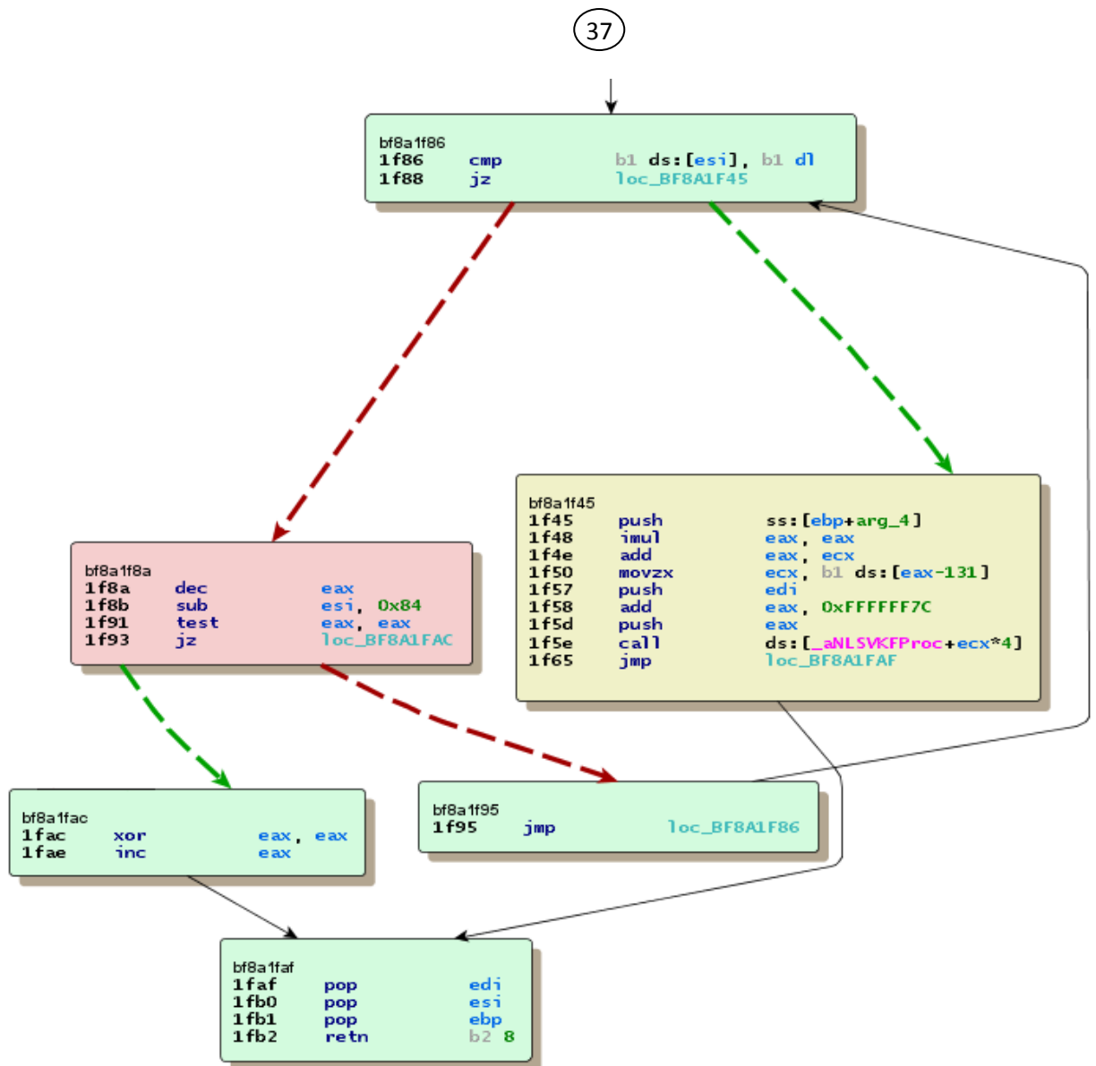
Figure 3.23 – A part of the xxxEKNLSProcs procedure before patching
